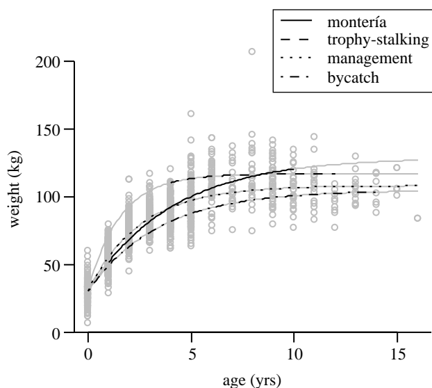
Figure 2. The relationship between age and weight for each hunting type considered in this study. The points represent empirical data while the lines show predictions for each hunting type from the nonlinear regression model (see table 1 for details). The ranges for which data are available are depicted with heavy lines, while areas for which we have no empirical data are shown with faint grey lines.
